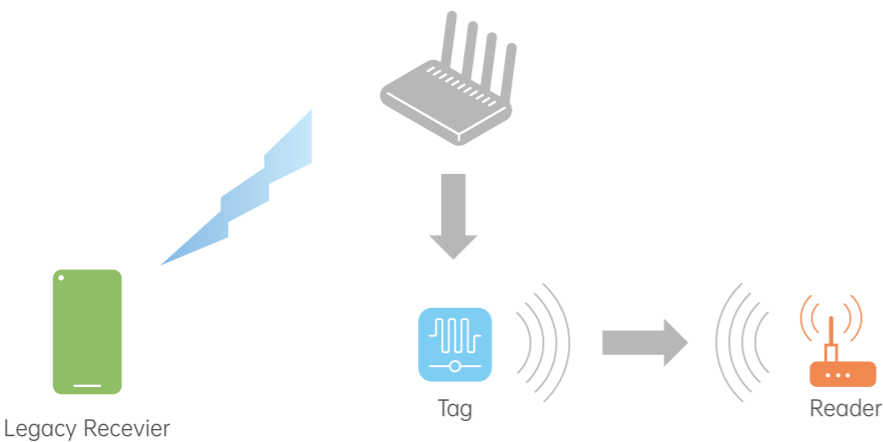
Figure 6.2-1 Illustration of Ambient Backscatter Communications system
