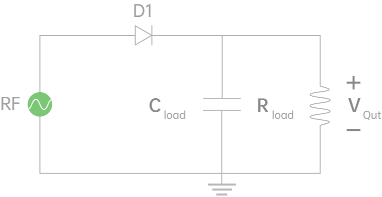
Figure 3.1-1 Half-wave rectifier
