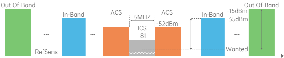
Figure 4.3-1 Rx requirements for coexistence
