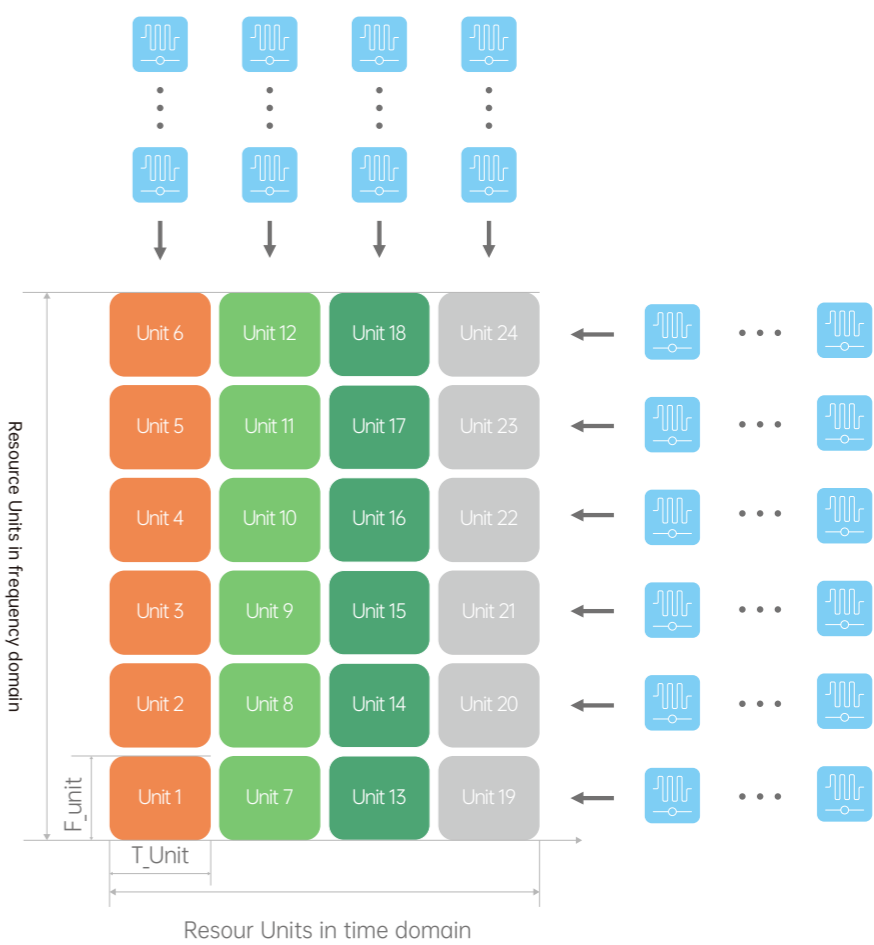
Figure 5.2-2 Resource allocation for Zero-Power communication
