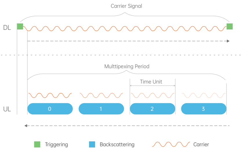
Figure 5.2-1 TDMA-based zero-power communication
