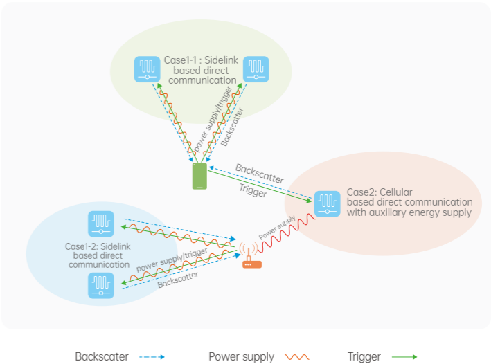
Figure 4.2-2 Sidelink based zero-power communication system
