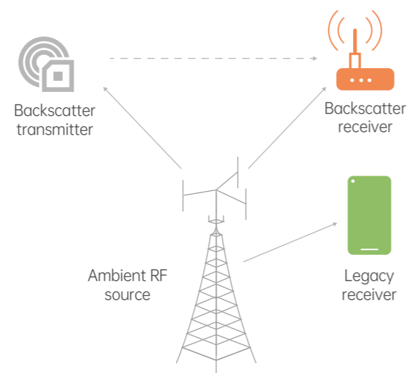
Figure 3.2-1 Illustration of AmBC system [6]
