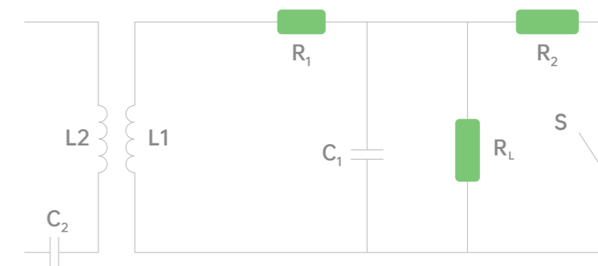
Figure 3.2-3 Resistance-based modulation
