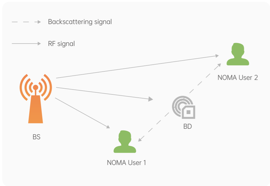
Figure 6.4-1 Downlink NOMA combined with backscatter: use a separate backscatter device
