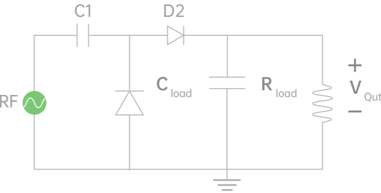
Figure 3.1-2 Single stage voltage multiplier
